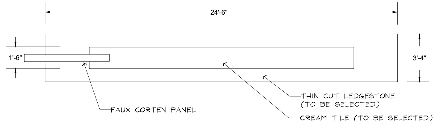
MONUMENT PLAN - (Double Sided Sign) 1/4"=1'-0"
